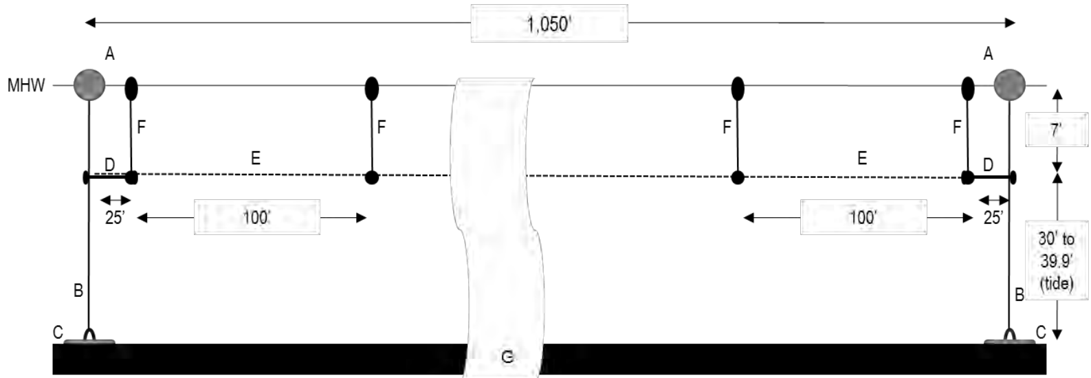
Chebeague Site Cross Section View- Not to Scale
